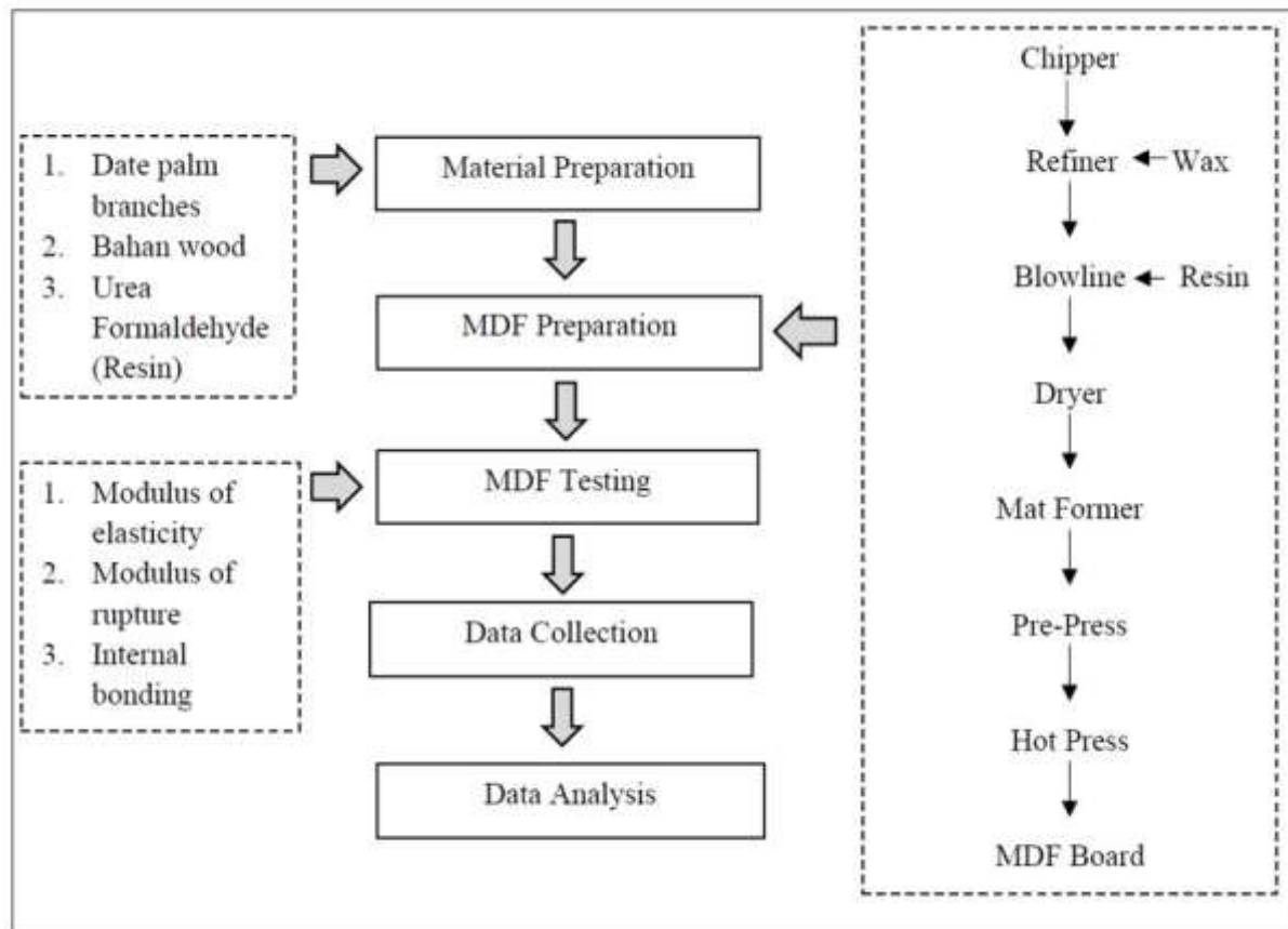
Figure 1. Methodology for producing MDF from admixture date palm branches and Bahan wood
