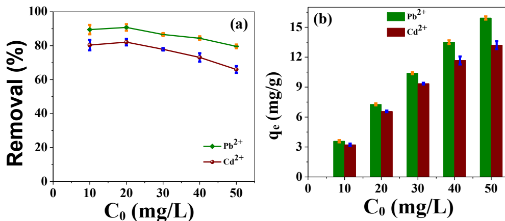
Figure 7. Effect of initial concentration on a) removal (%) and b) adsorption capacity ( q_e ) of \text{Pb}^{2+} & \text{Cd}^{2+} on the NC. Conditions: 0.125 g of NC; 50.0 mL ion solution; at optimal conditions for pH and contact time.
