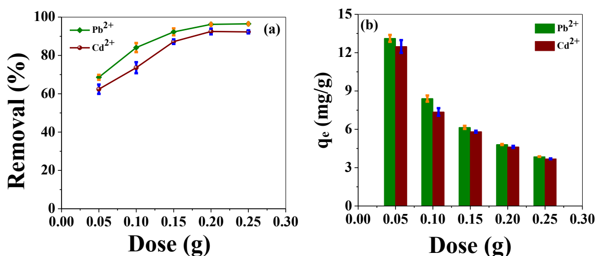
Figure 8. Effect of NC dose on a) the removal (%) and b) the adsorption capacity ( q_e ) of \text{Pb}^{2+} and \text{Cd}^{2+} onto the NC. Conditions: 50.0 mL \text{Cd}^{2+} solution at optimal conditions for pH, contact time, and initial concentration.
